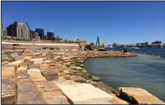
Sandstone placement along western foreshore
