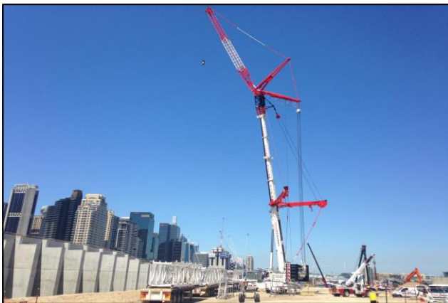
350t Liebherr Mobile Crane Installation
